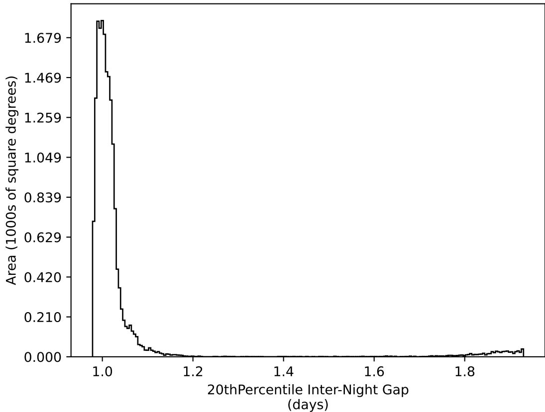
baseline_v3.5_10yrs WFD all bands: 20thPercentile Inter-Night Gap
