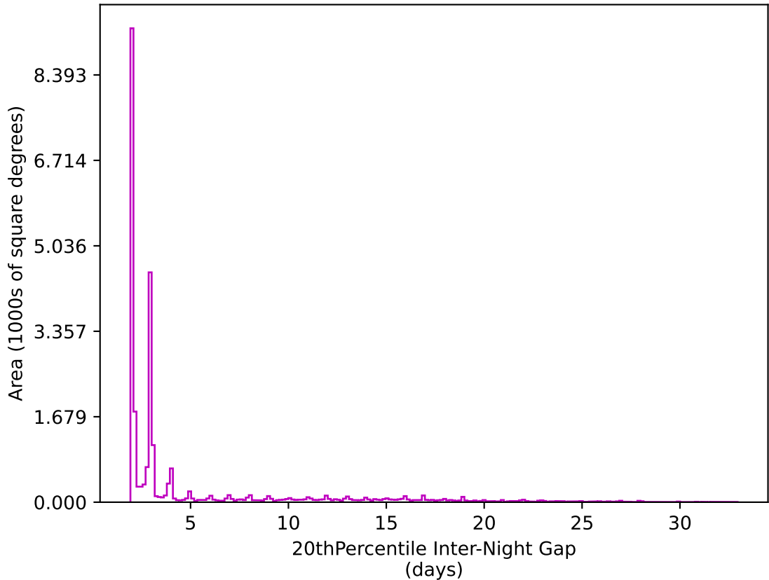
baseline_v3.5_10yrs All sky z band: 20thPercentile Inter-Night Gap
