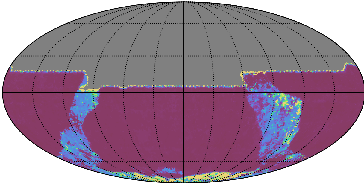
baseline_v3.5_10yrs All sky y band: 20thPercentile Inter-Night Gap
