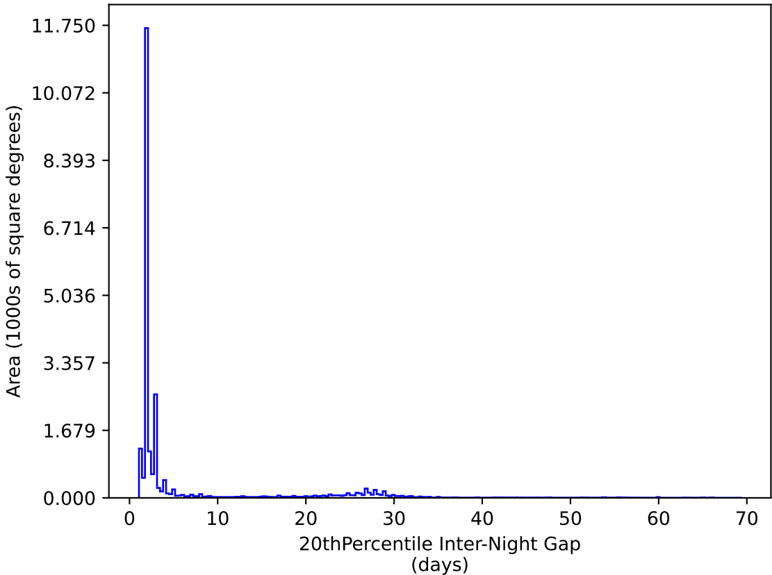
baseline_v3.5_10yrs All sky y band: 20thPercentile Inter-Night Gap
