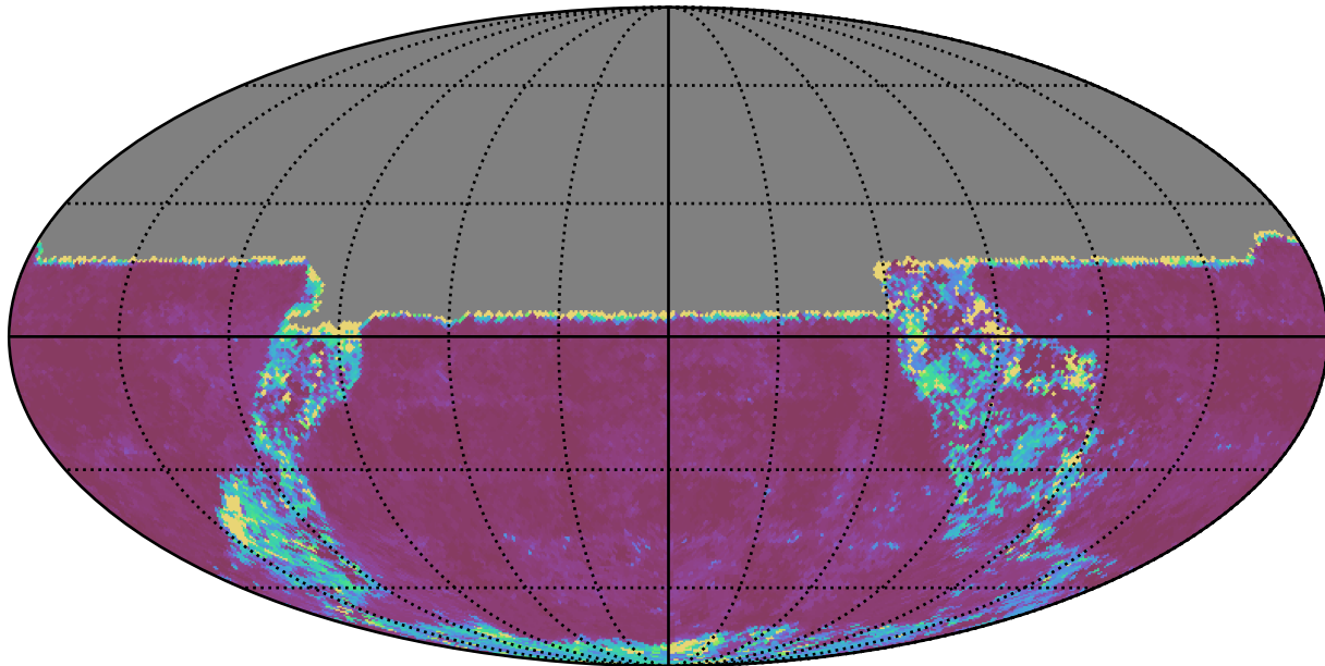
baseline_v3.5_10yrs All sky u band: 20thPercentile Inter-Night Gap
