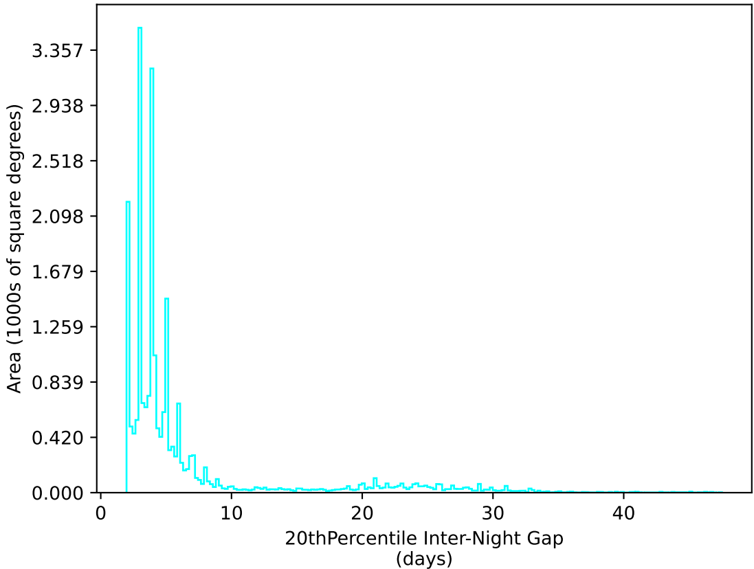
baseline_v3.5_10yrs All sky u band: 20thPercentile Inter-Night Gap
