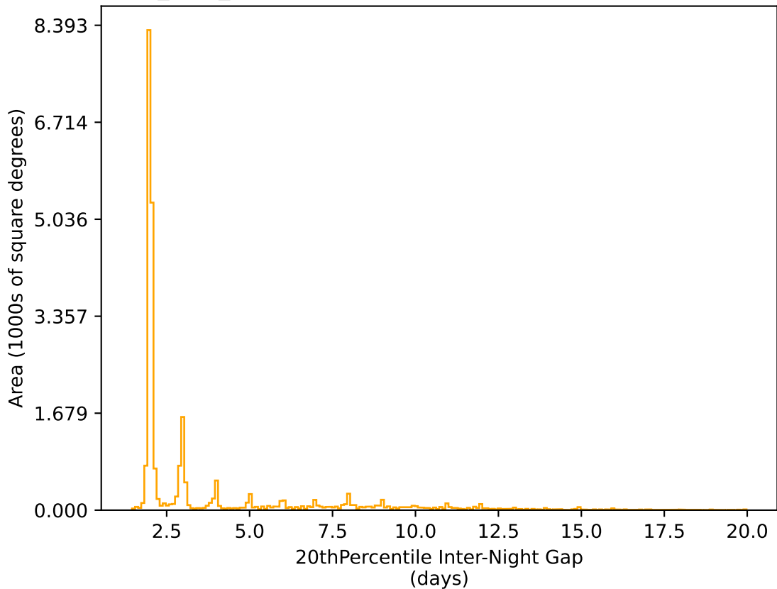
baseline_v3.5_10yrs All sky r band: 20thPercentile Inter-Night Gap
