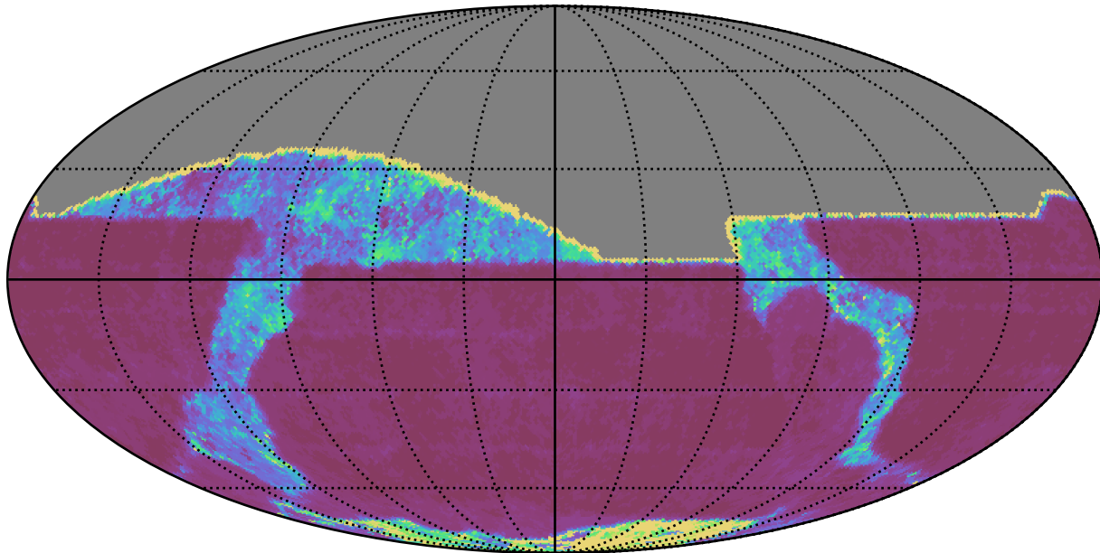
baseline_v3.5_10yrs All sky i band: 20thPercentile Inter-Night Gap
