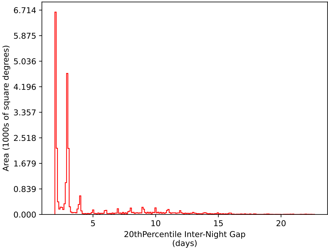
baseline_v3.5_10yrs All sky i band: 20thPercentile Inter-Night Gap
