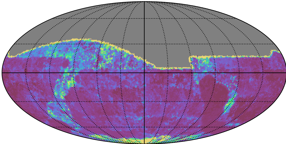
baseline_v3.5_10yrs All sky g band: 20thPercentile Inter-Night Gap
