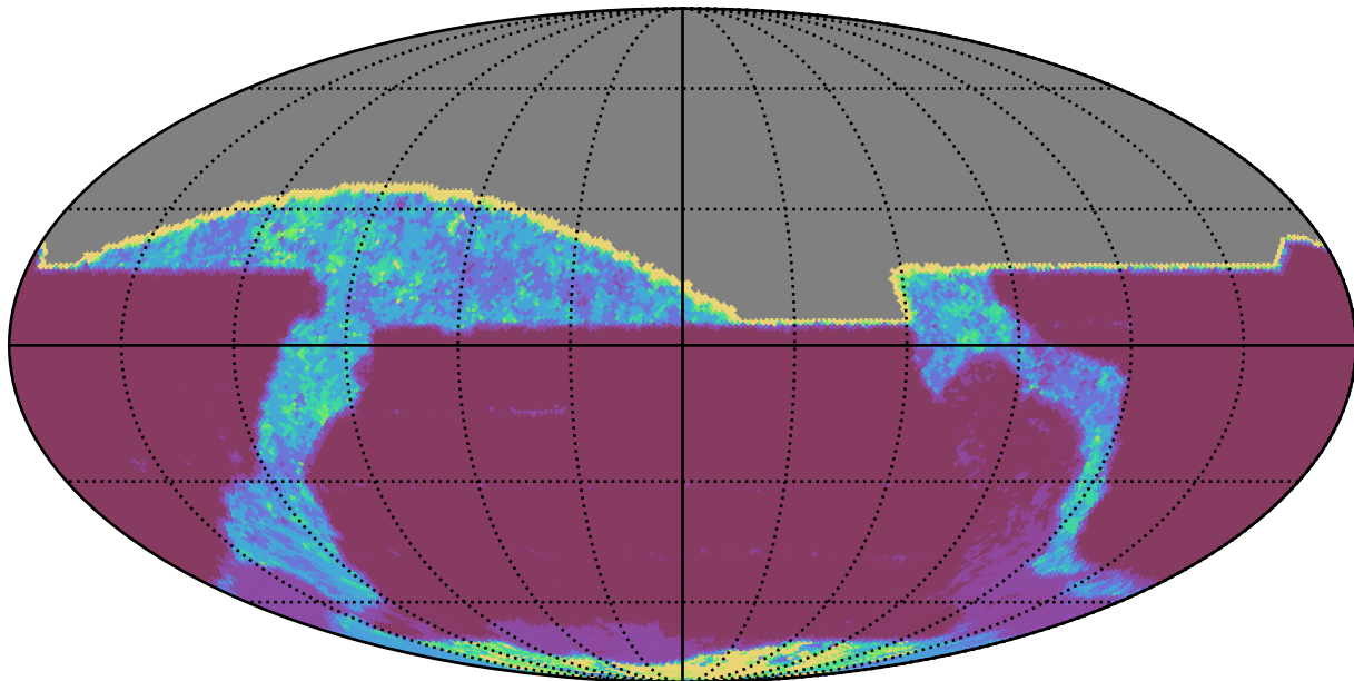
baseline_v3.5_10yrs All sky all bands: 20thPercentile Inter-Night Gap
