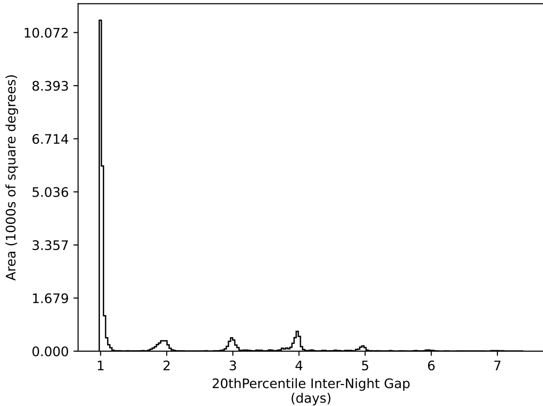
baseline_v3.5_10yrs All sky all bands: 20thPercentile Inter-Night Gap
