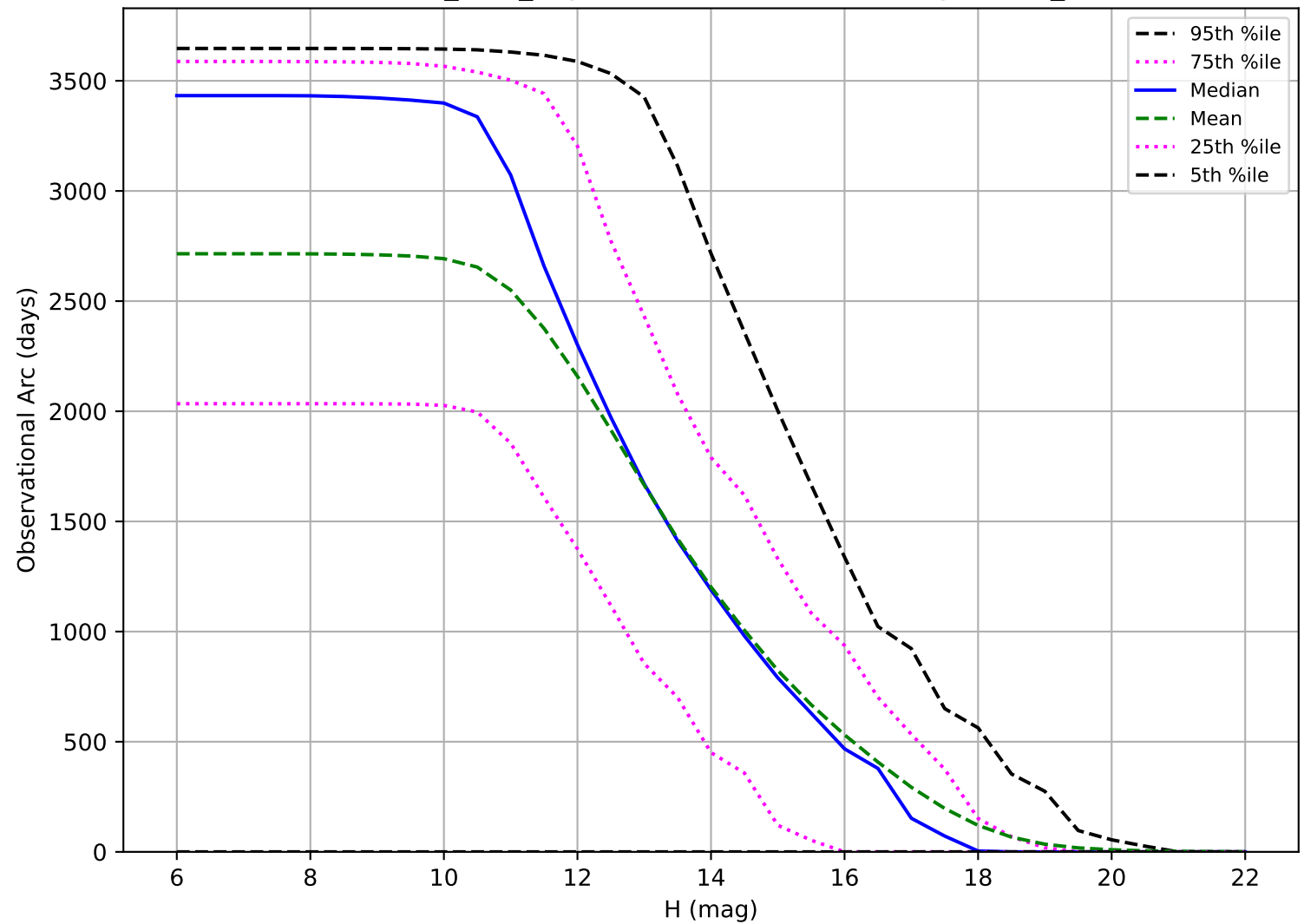
baseline_v3.4_10yrs: Observational Arc Length OCC_r5
