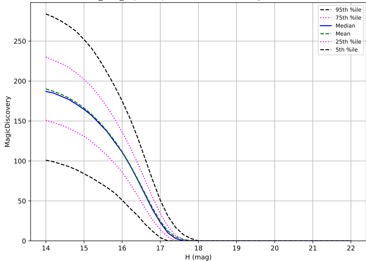
baseline_v3.4_10yrs: Trojan 6 detections in 60 nights detection loss
