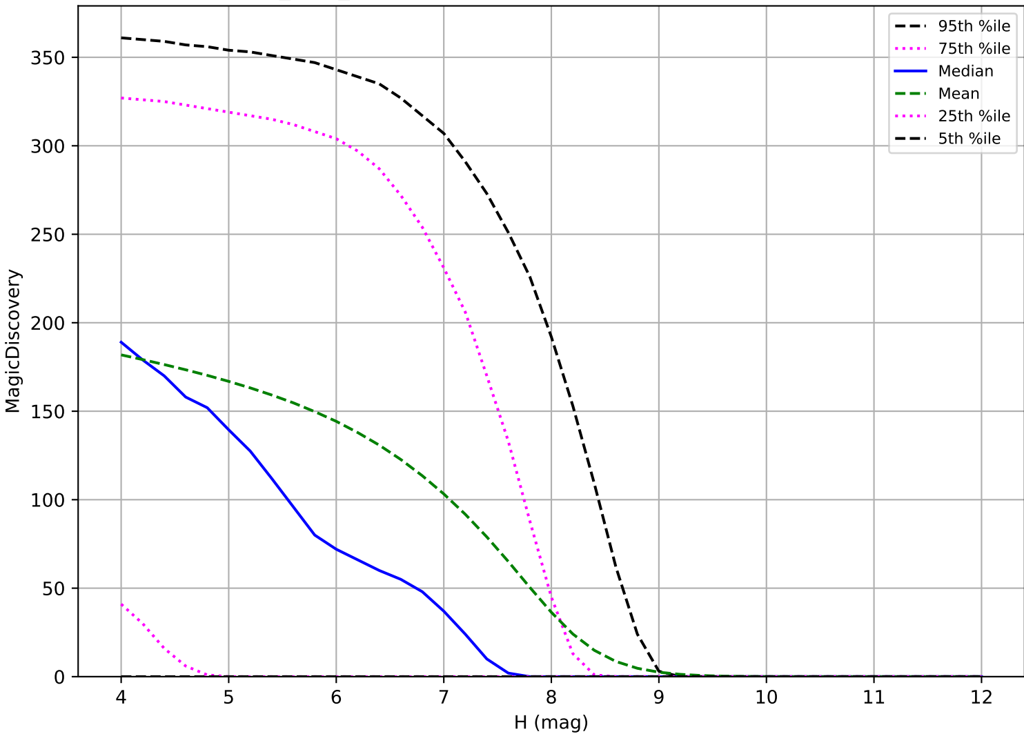
baseline_v3.4_10yrs: TNO 6 detections in 60 nights detection loss
