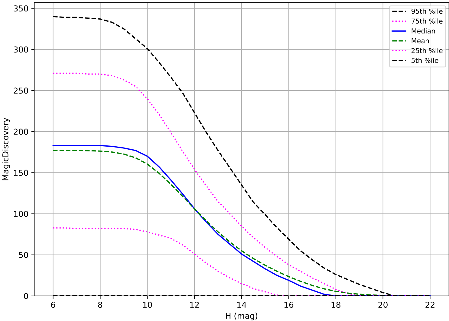
baseline_v3.4_10yrs: OCC_r5 6 detections in 60 nights detection loss
