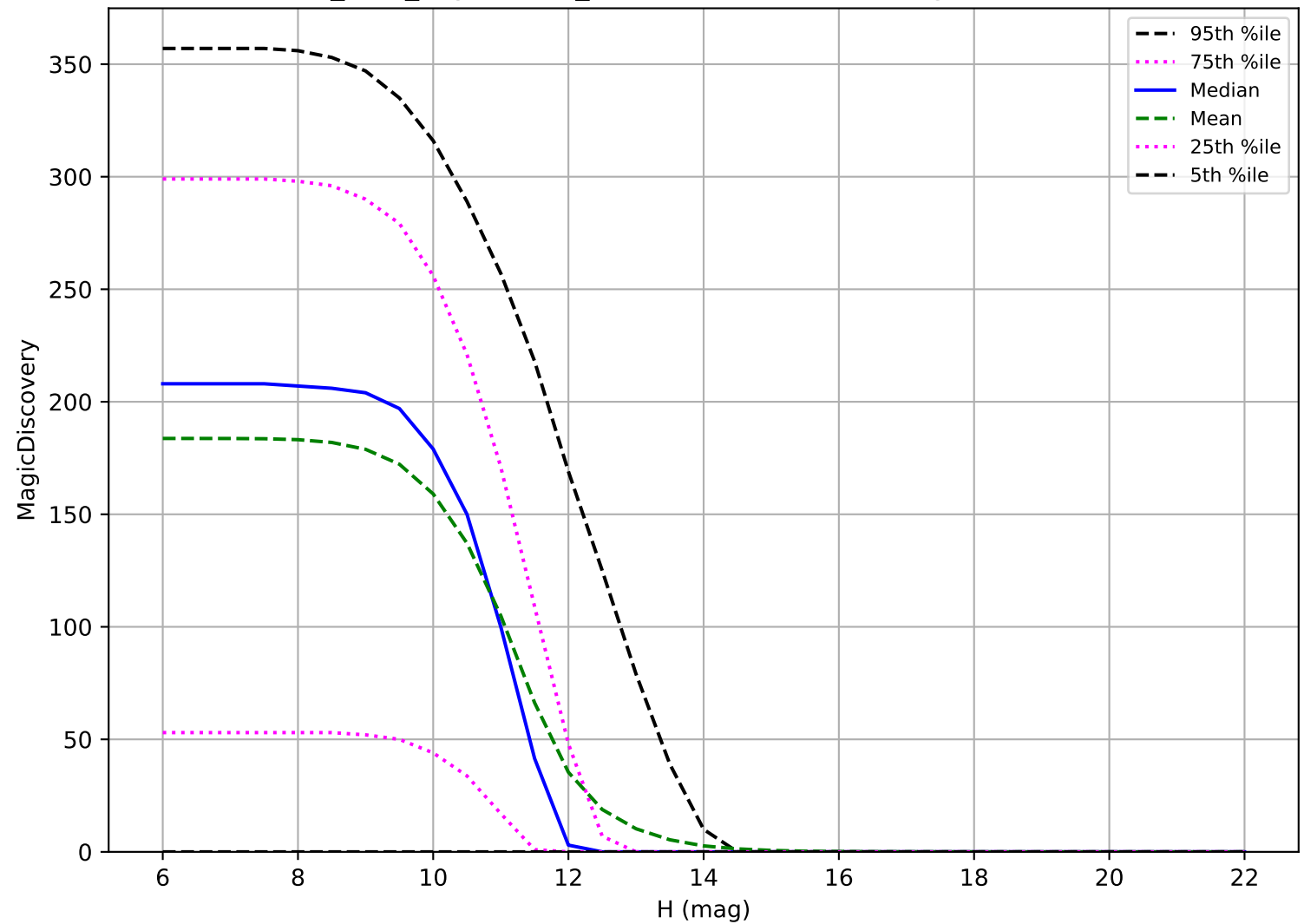
baseline_v3.4_10yrs: OCC_r20 6 detections in 60 nights detection loss
