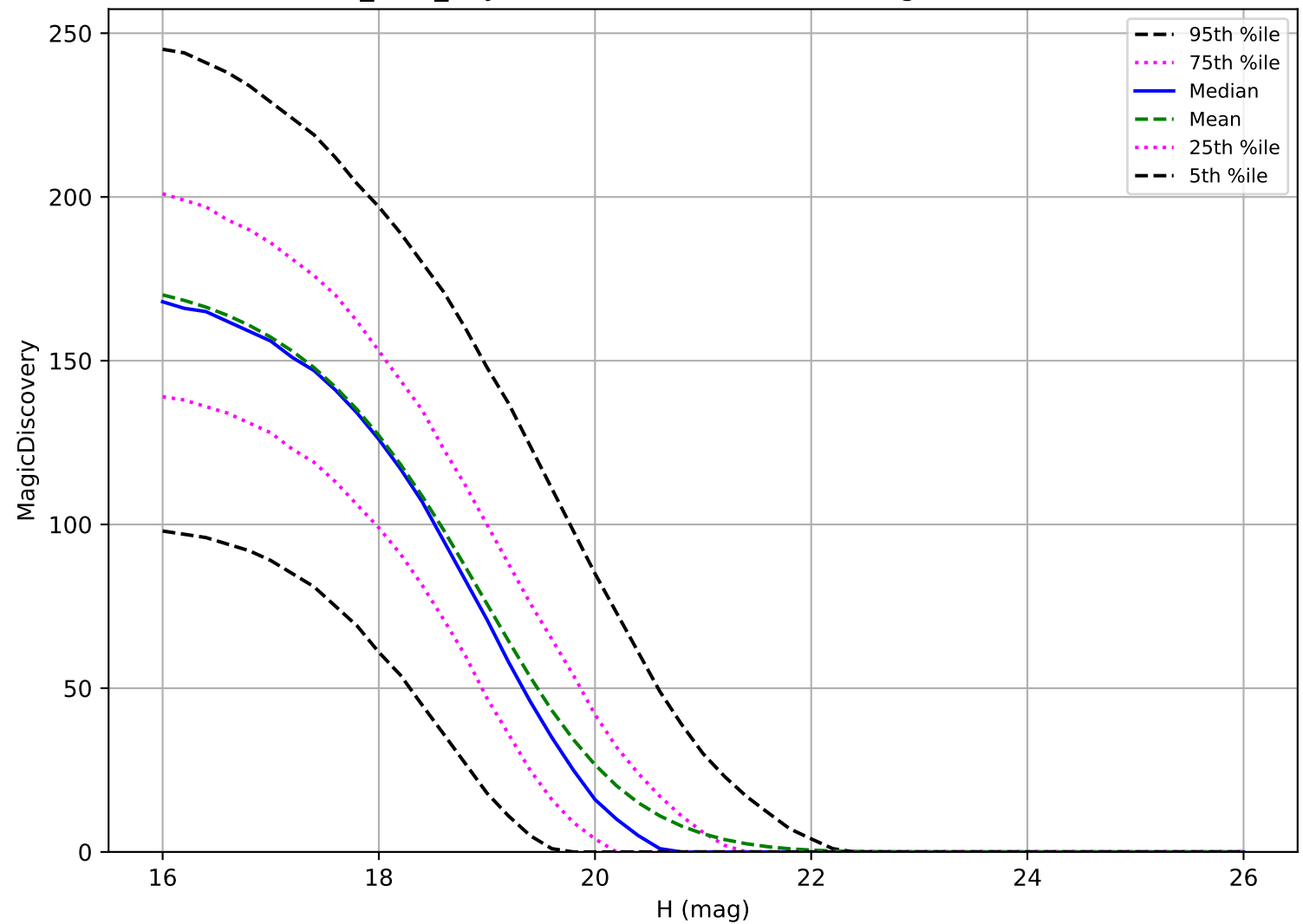
baseline_v3.4_10yrs: MBA 6 detections in 60 nights detection loss
