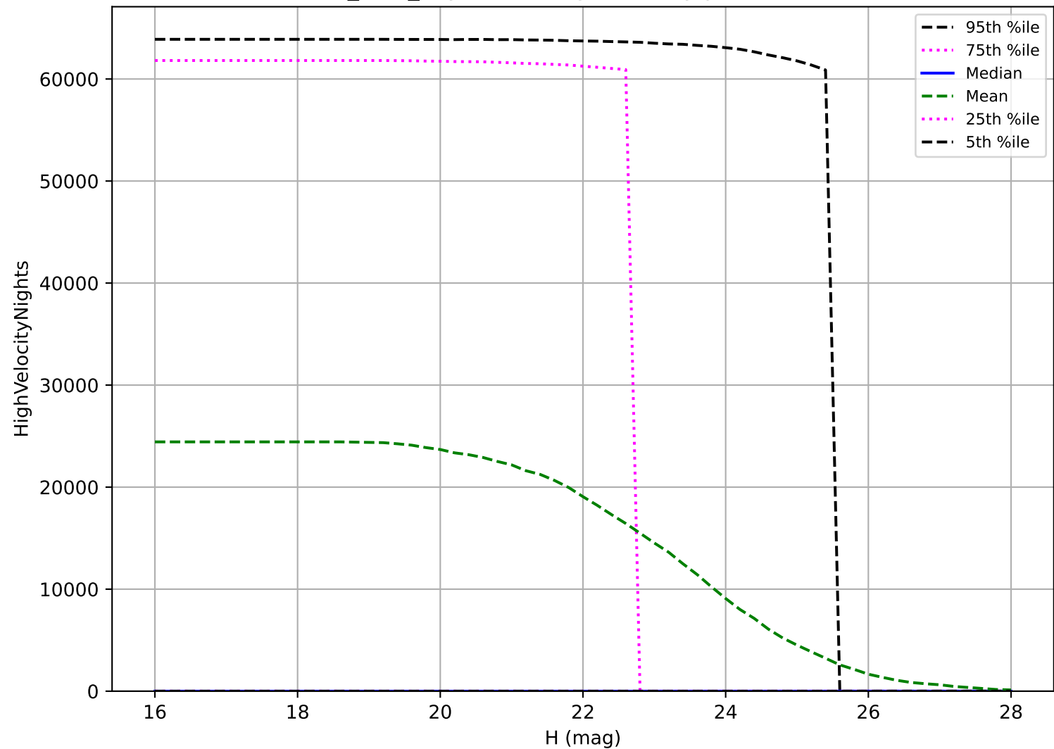
baseline_v3.4_10yrs: PHA High velocity pair detection loss
