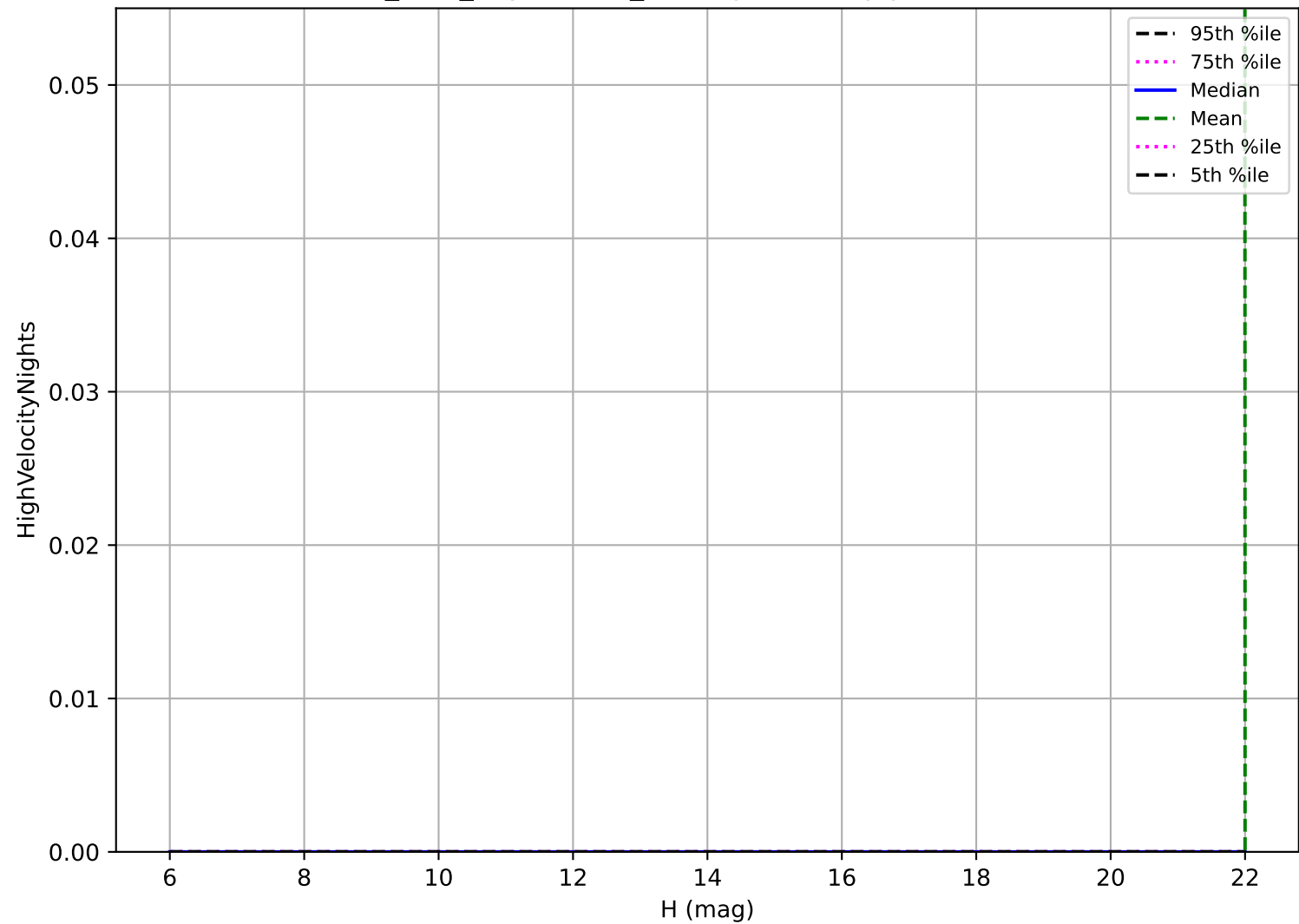
baseline_v3.4_10yrs: OCC_r20 High velocity pair detection loss
