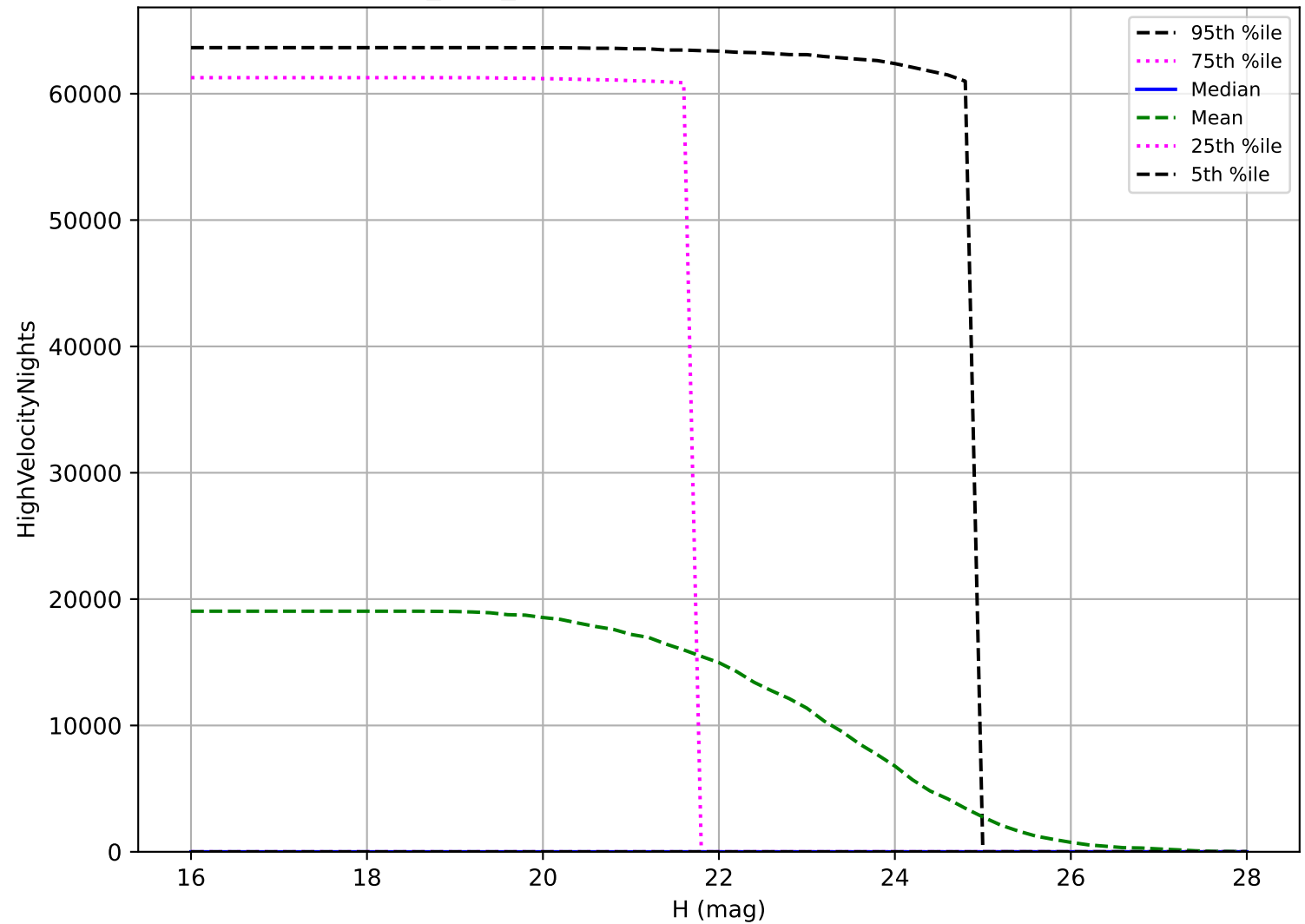
baseline_v3.4_10yrs: NEO High velocity pair detection loss
