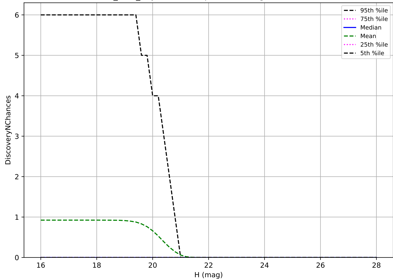
baseline_v3.4_10yrs: Vatira 3 pairs in 15 nights detection loss
