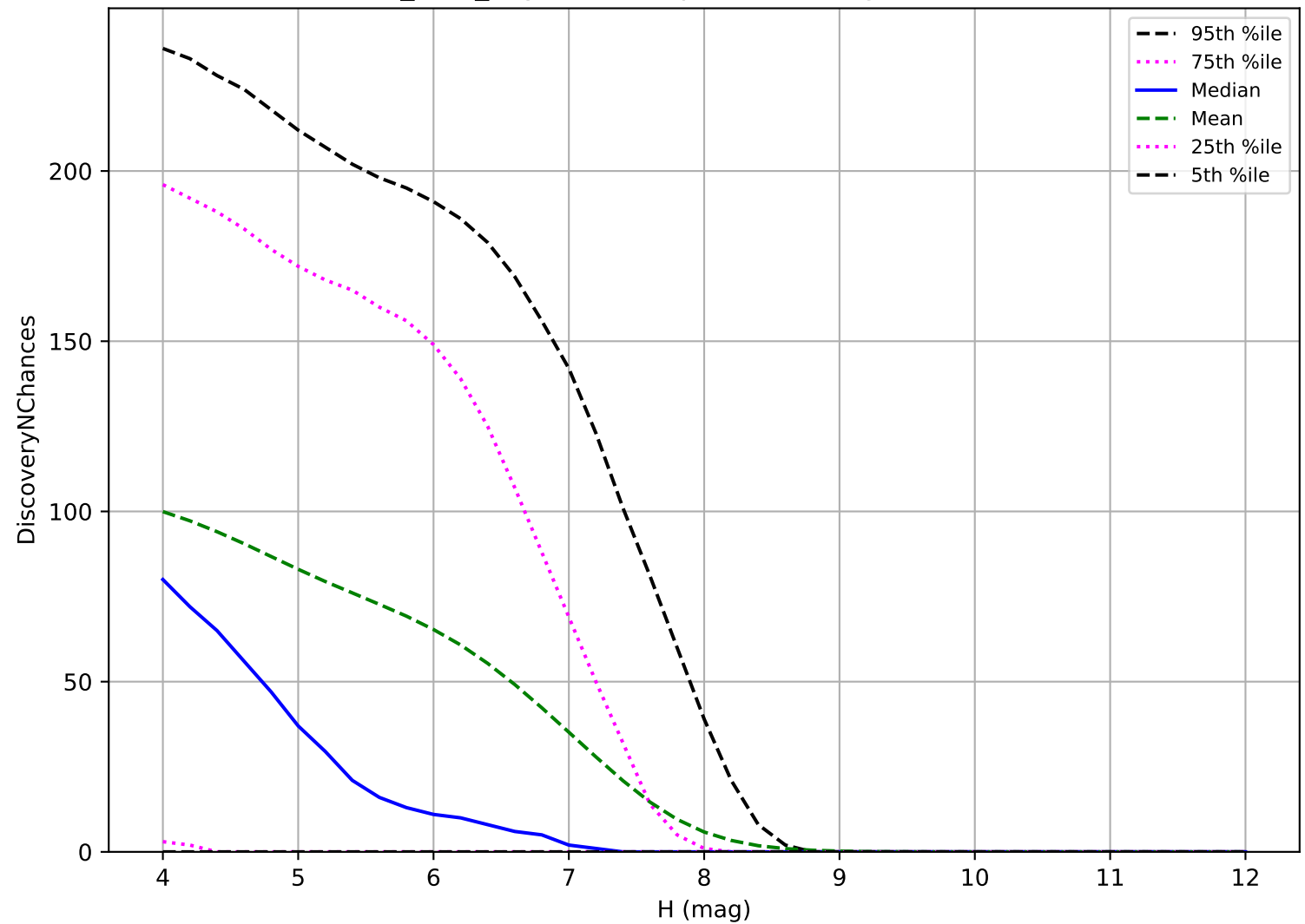
baseline_v3.4_10yrs: TNO 3 pairs in 15 nights detection loss
