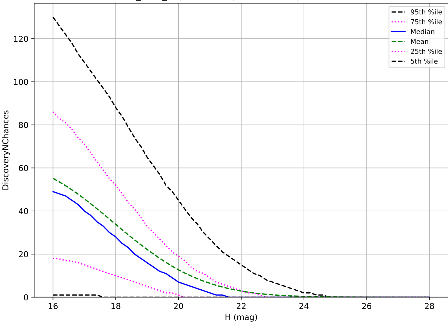
baseline_v3.4_10yrs: PHA 3 pairs in 15 nights detection loss
