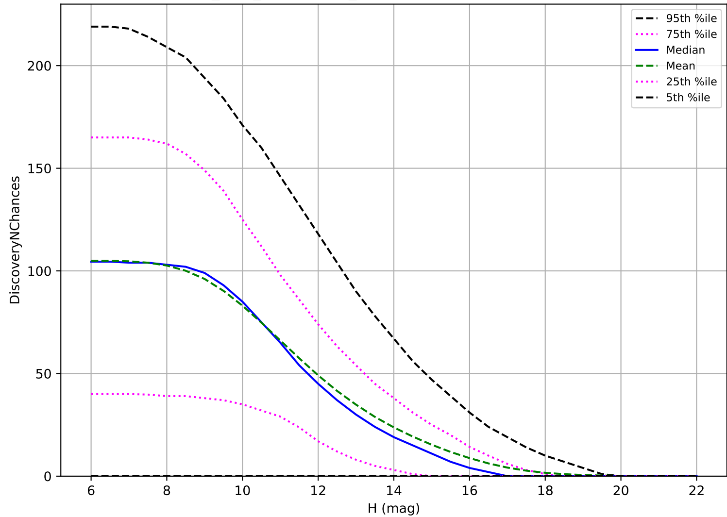
baseline_v3.4_10yrs: OCC_r5 3 pairs in 15 nights detection loss
