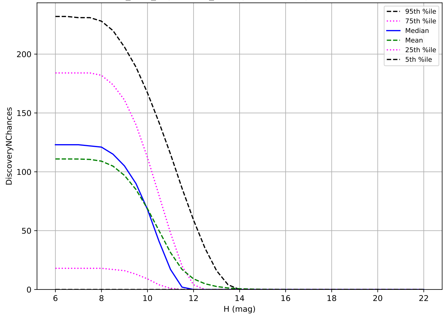
baseline_v3.4_10yrs: OCC_r20 3 pairs in 15 nights detection loss
