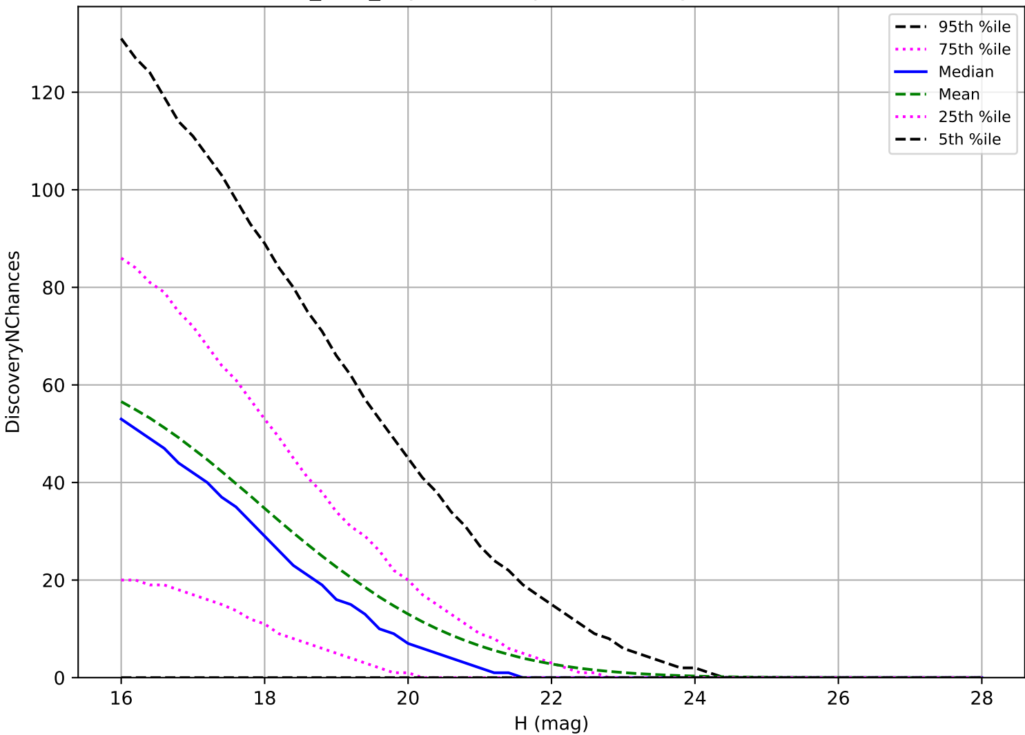
baseline_v3.4_10yrs: NEO 3 pairs in 15 nights detection loss
