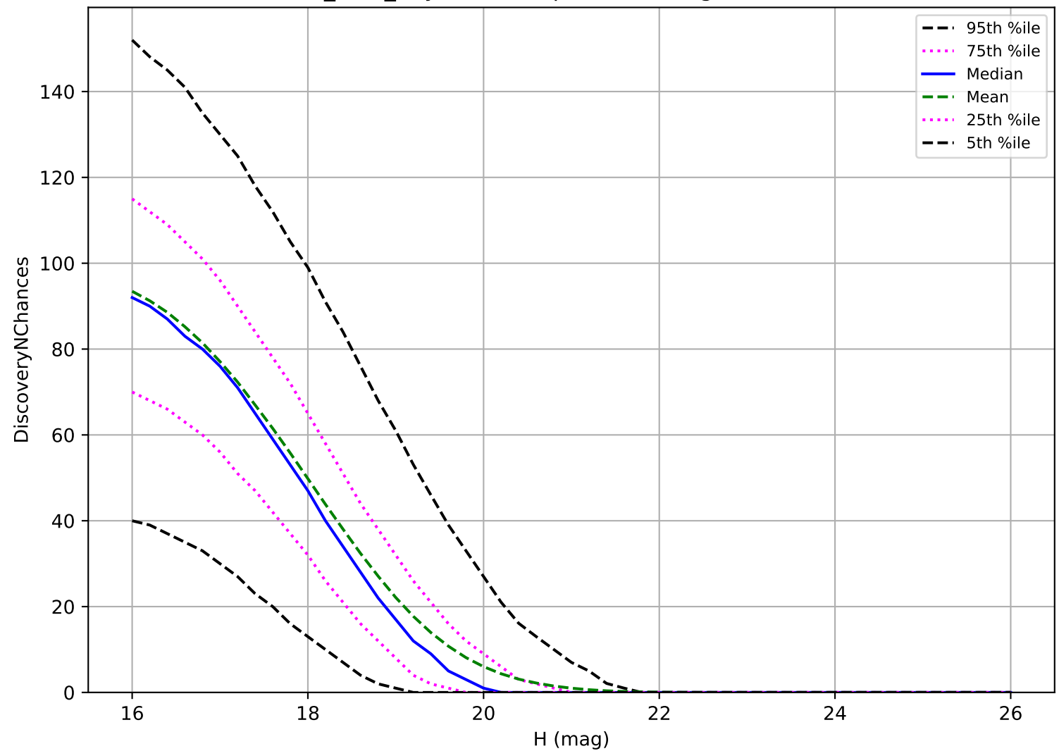
baseline_v3.4_10yrs: MBA 3 pairs in 15 nights detection loss
