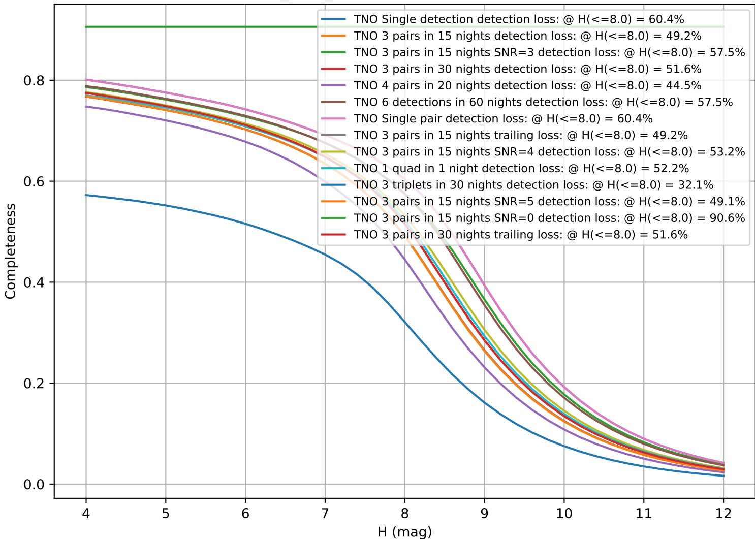
baseline_v3.4_10yrs: CumulativeCompleteness
