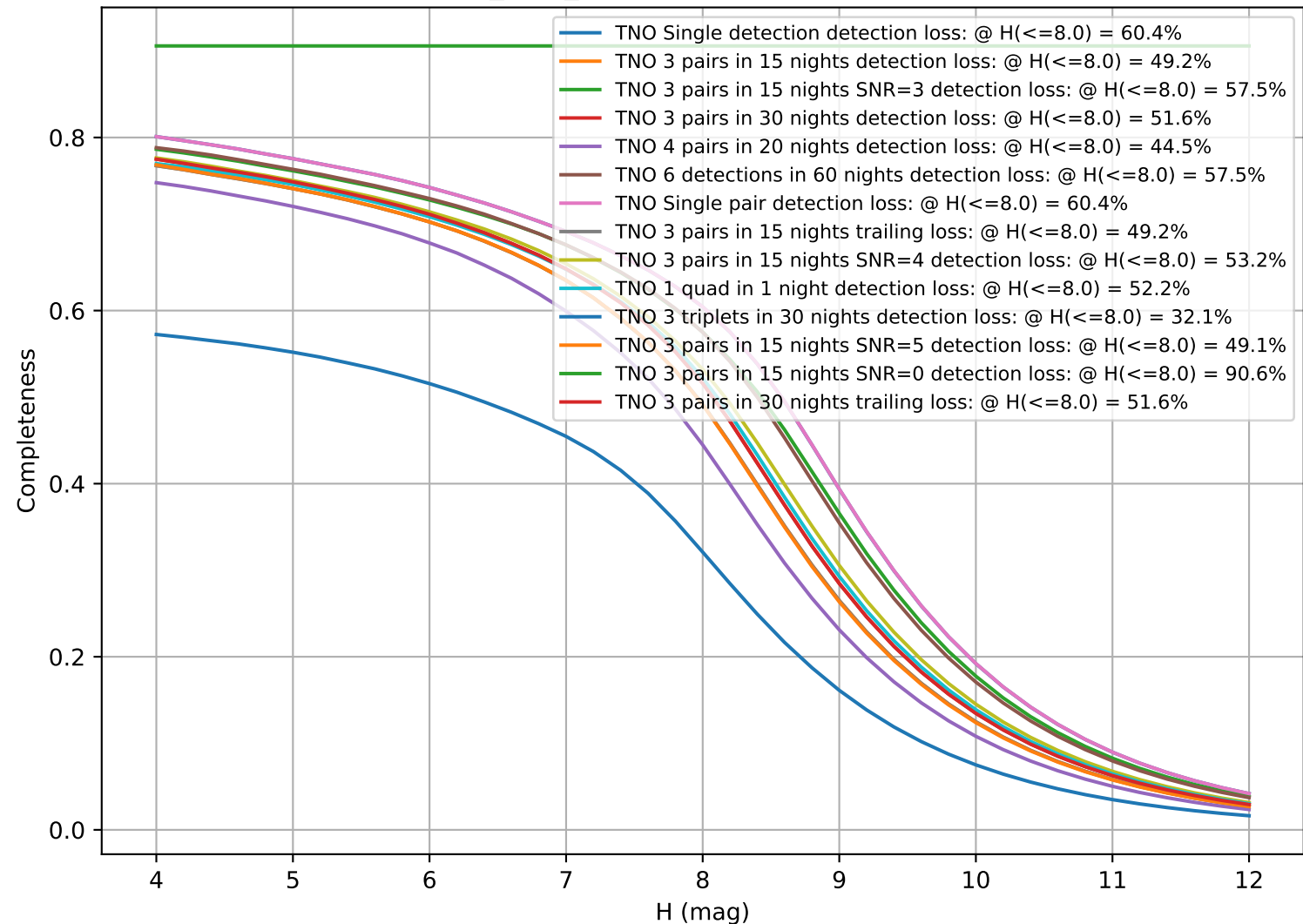
baseline_v3.4_10yrs: CumulativeCompleteness
