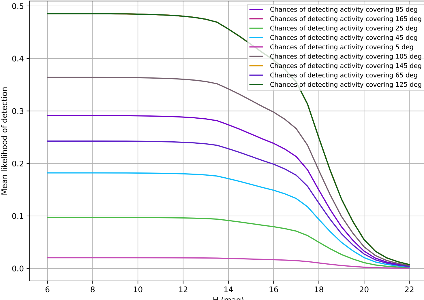
baseline_v3.4_10yrs OCC_r5
