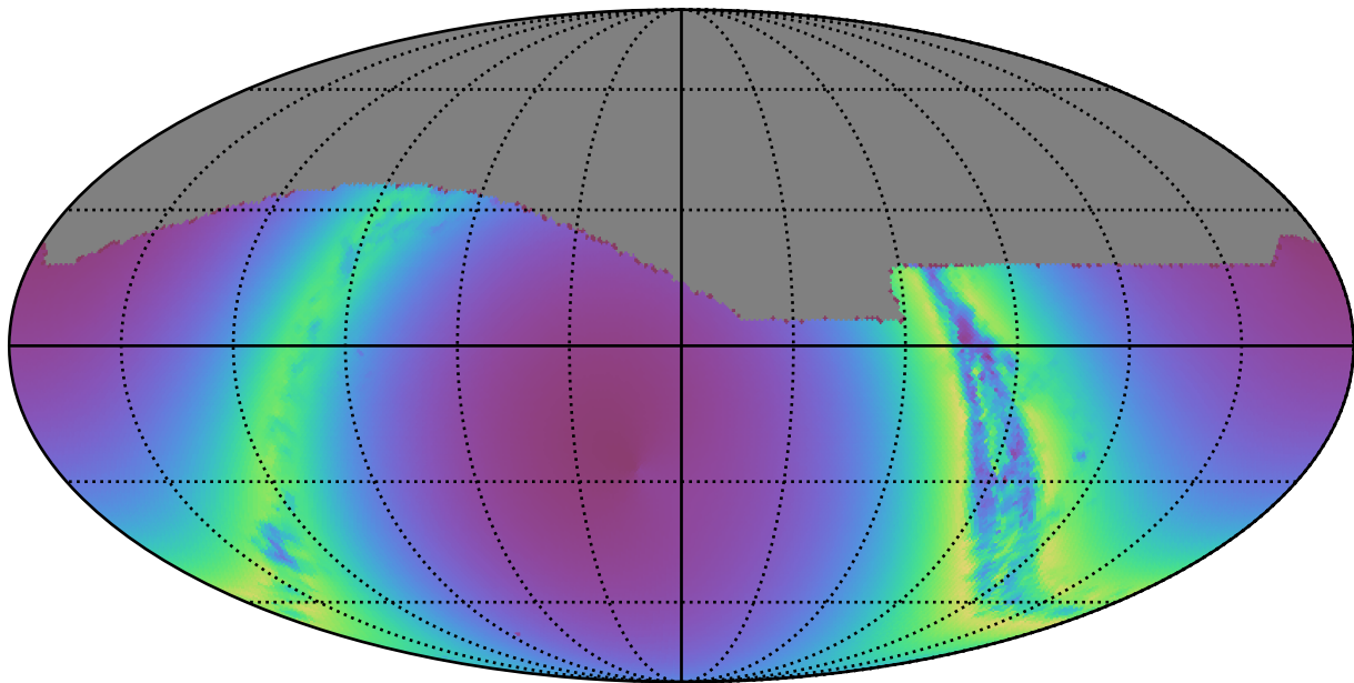
baseline_v3.4_10yrs : young_stars
