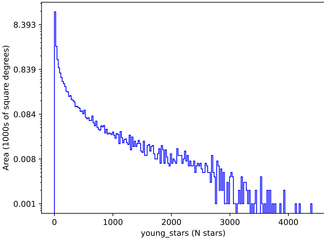
baseline_v3.4_10yrs : young_stars
