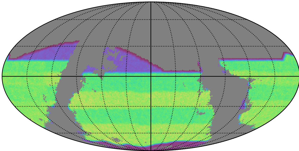
baseline_v3.4_10yrs gri band non-DD: riz_exposure_time_year9
