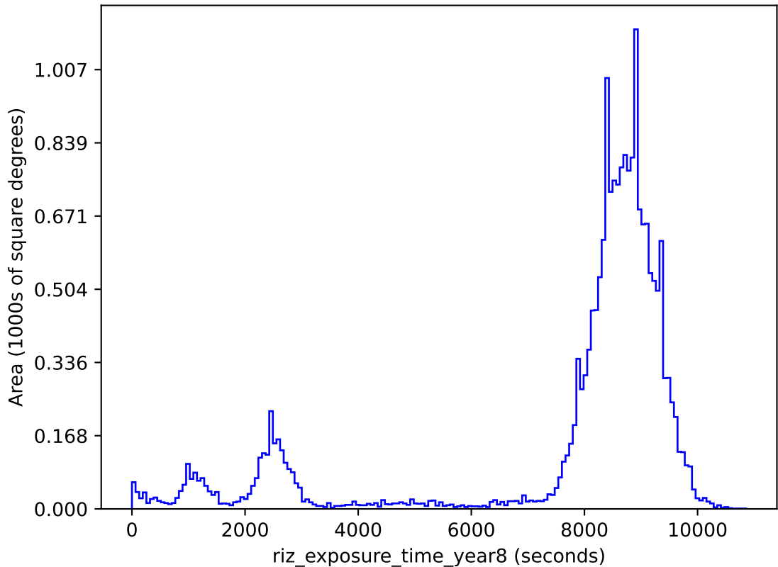
baseline_v3.4_10yrs gri band non-DD: riz_exposure_time_year8
