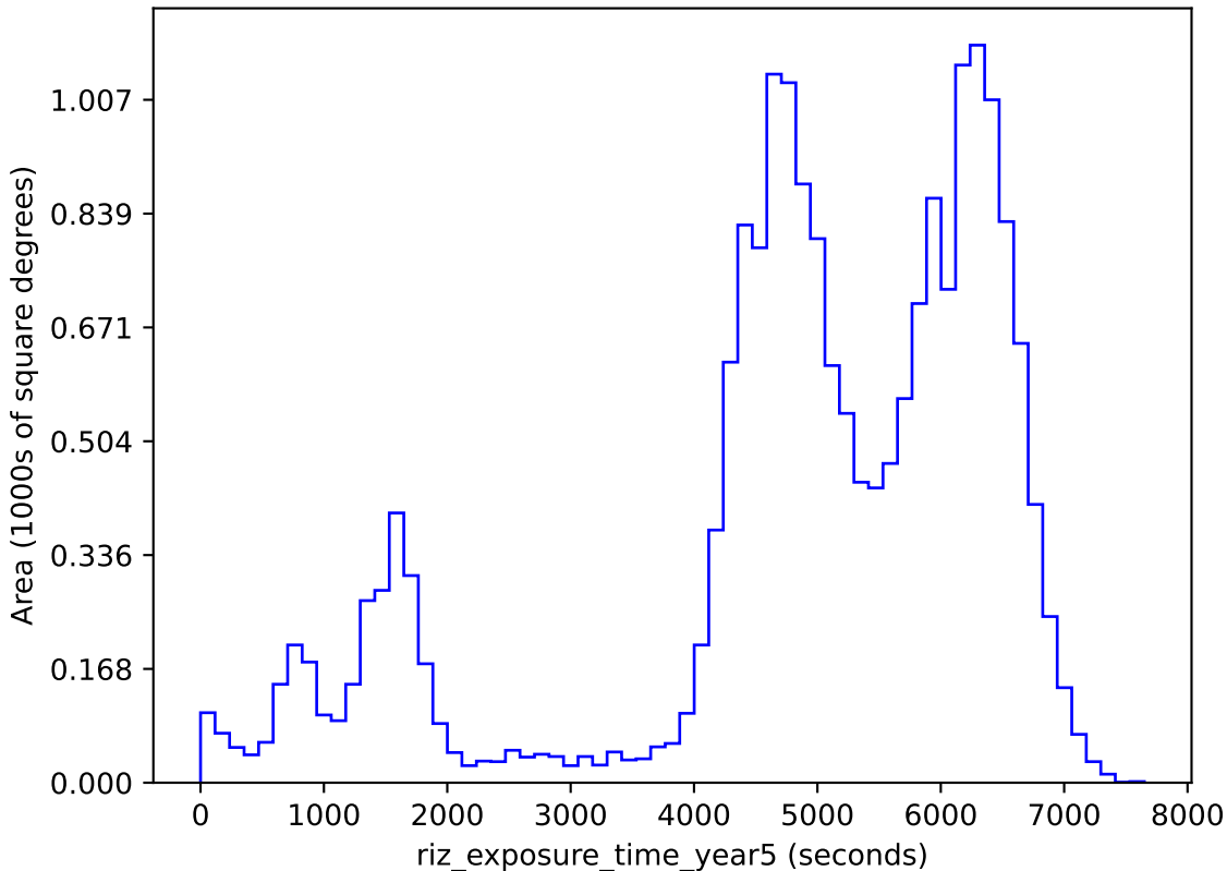
baseline_v3.4_10yrs gri band non-DD: riz_exposure_time_year5
