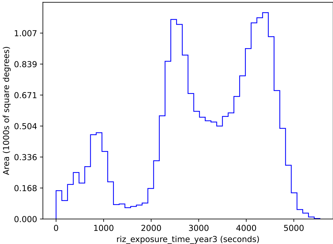
baseline_v3.4_10yrs gri band non-DD: riz_exposure_time_year3
