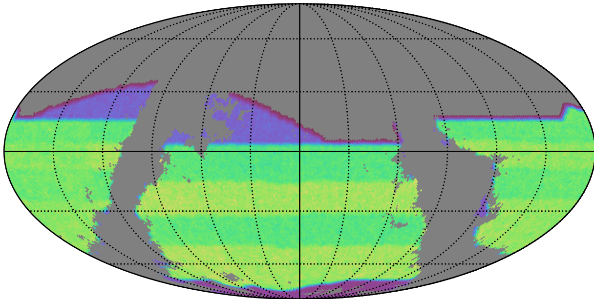
baseline_v3.4_10yrs gri band non-DD: gri_exposure_time_year9
