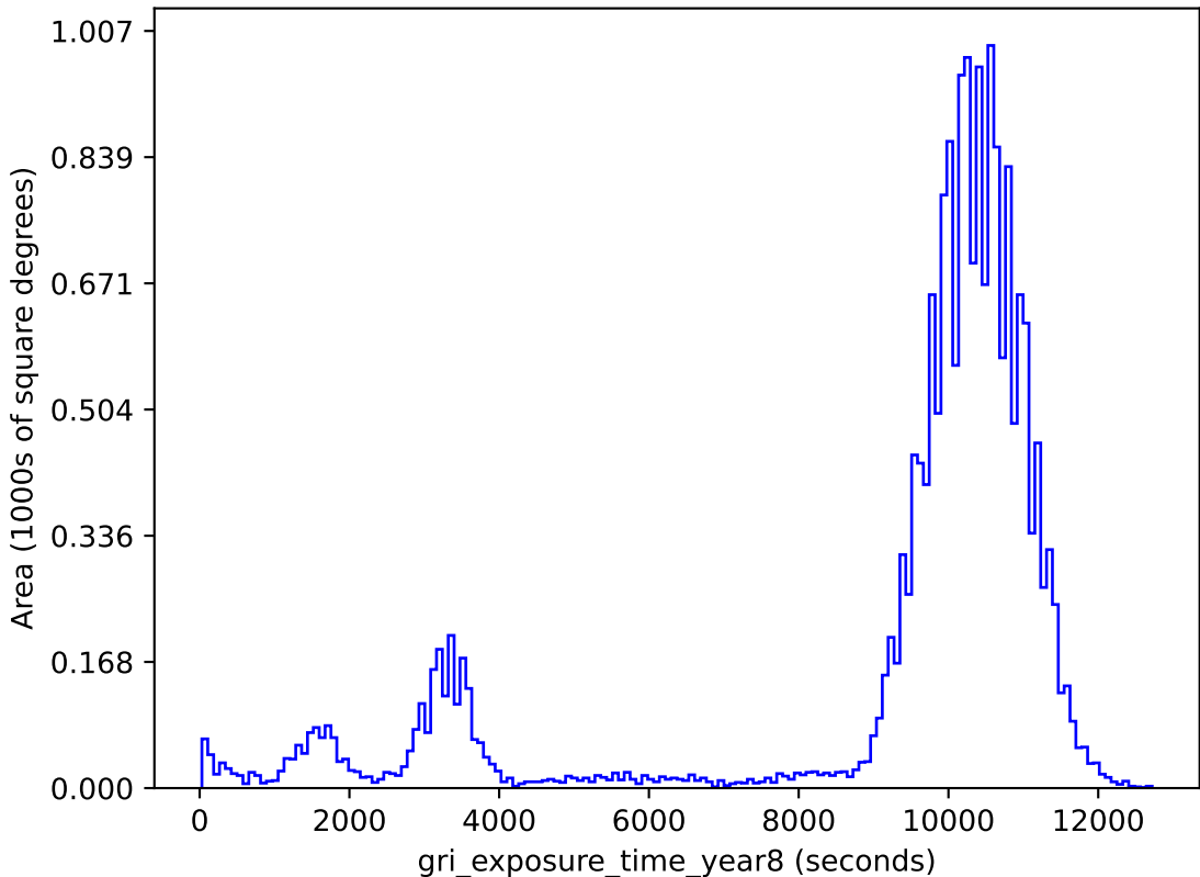
baseline_v3.4_10yrs gri band non-DD: gri_exposure_time_year8
