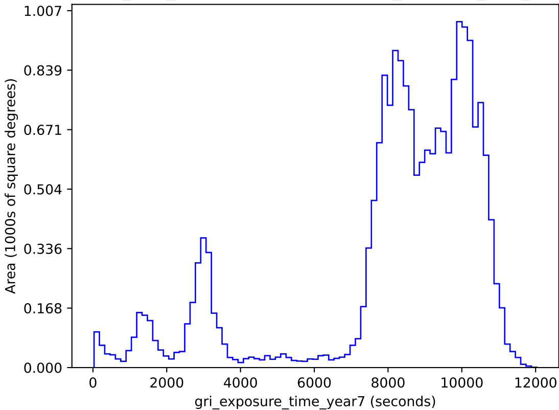
baseline_v3.4_10yrs gri band non-DD: gri_exposure_time_year7
