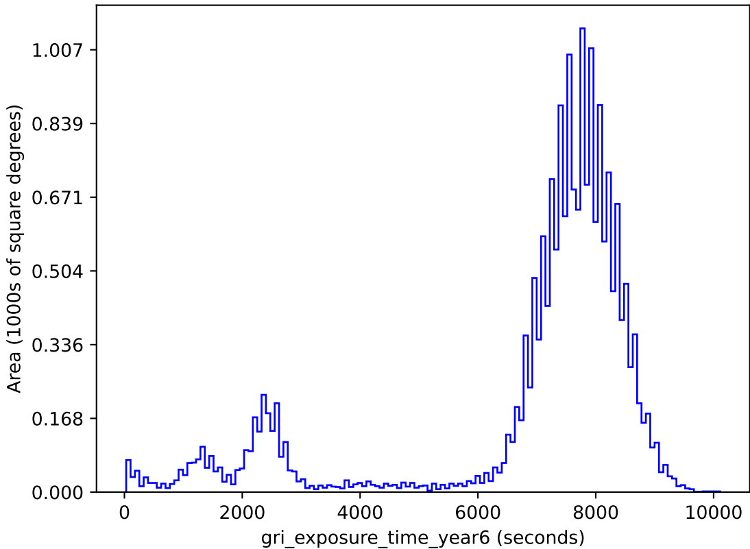
baseline_v3.4_10yrs gri band non-DD: gri_exposure_time_year6
