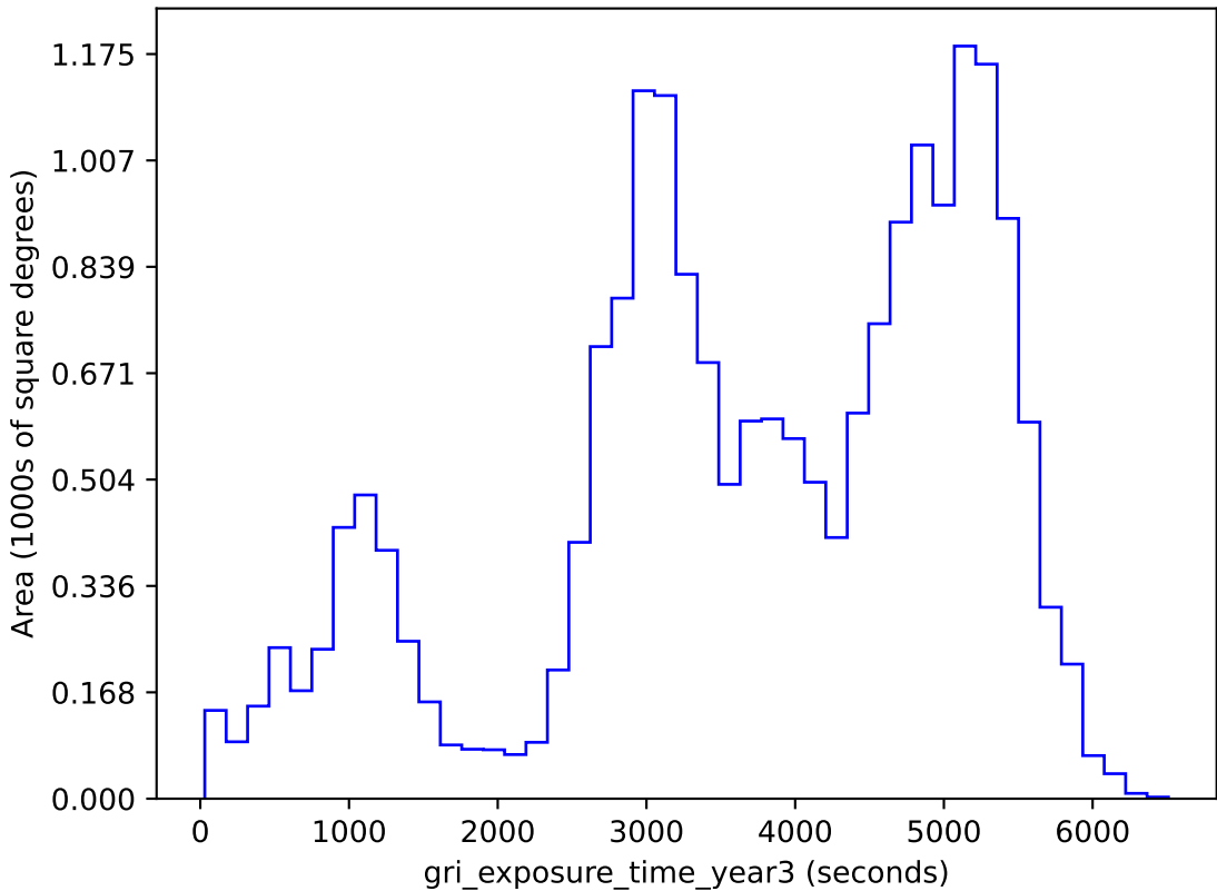
baseline_v3.4_10yrs gri band non-DD: gri_exposure_time_year3
