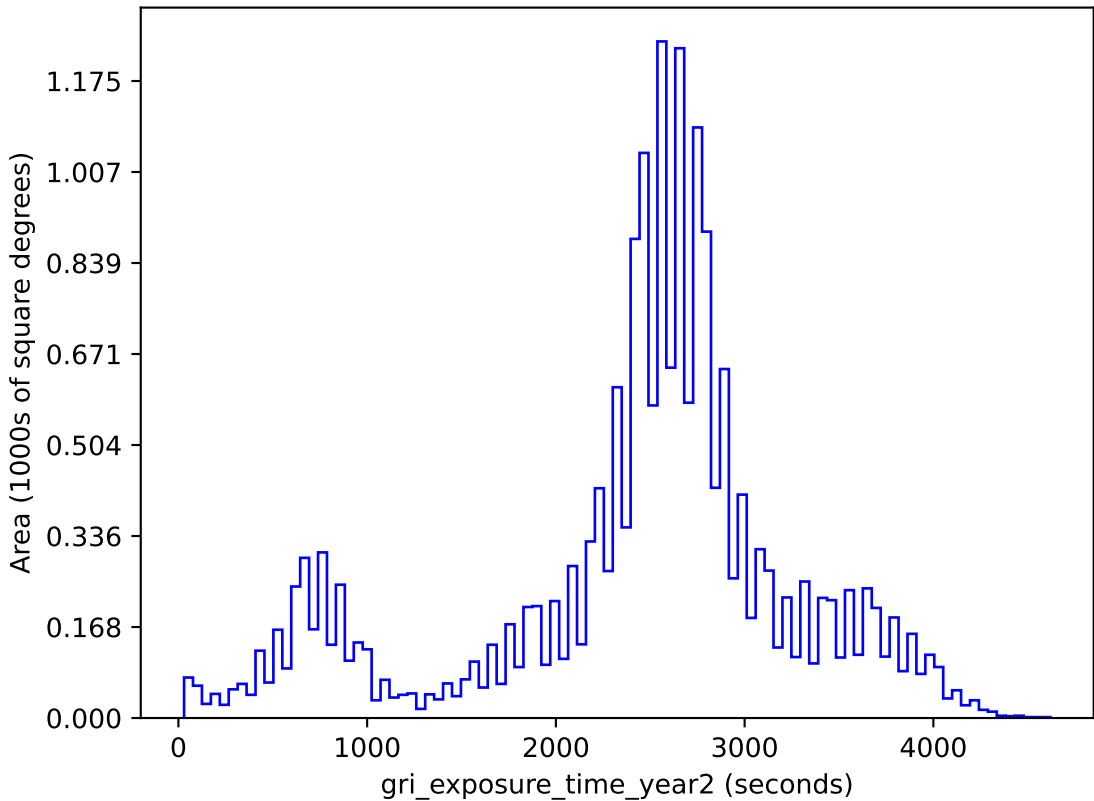
baseline_v3.4_10yrs gri band non-DD: gri_exposure_time_year2
