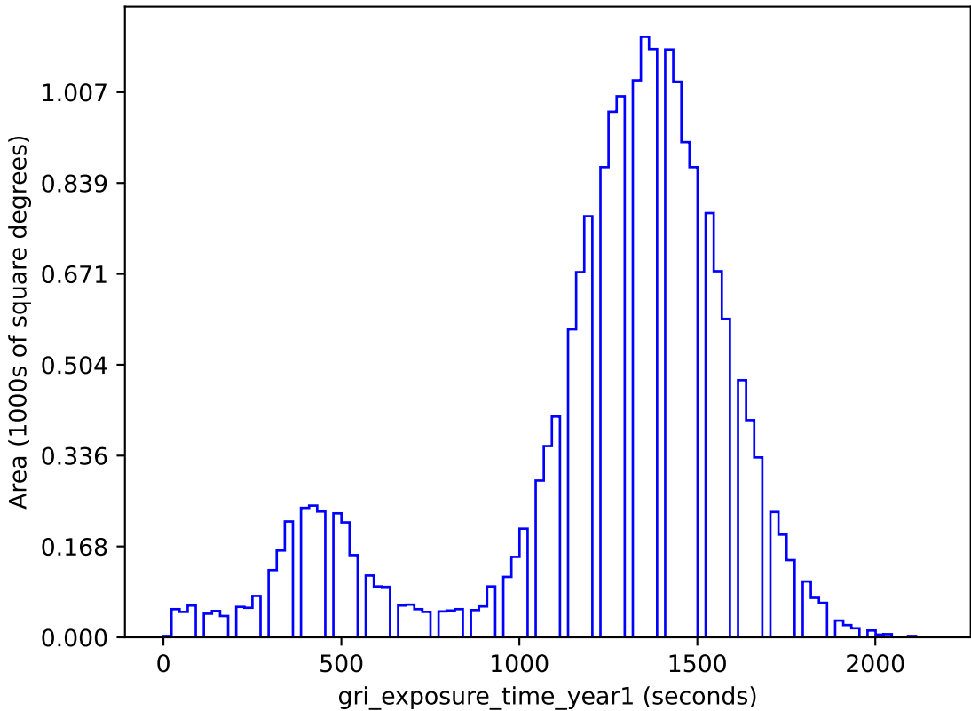
baseline_v3.4_10yrs gri band non-DD: gri_exposure_time_year1
