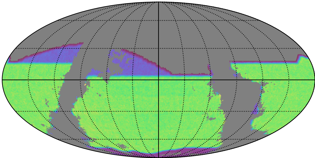
baseline_v3.4_10yrs gri band non-DD: gri_exposure_time_year10
