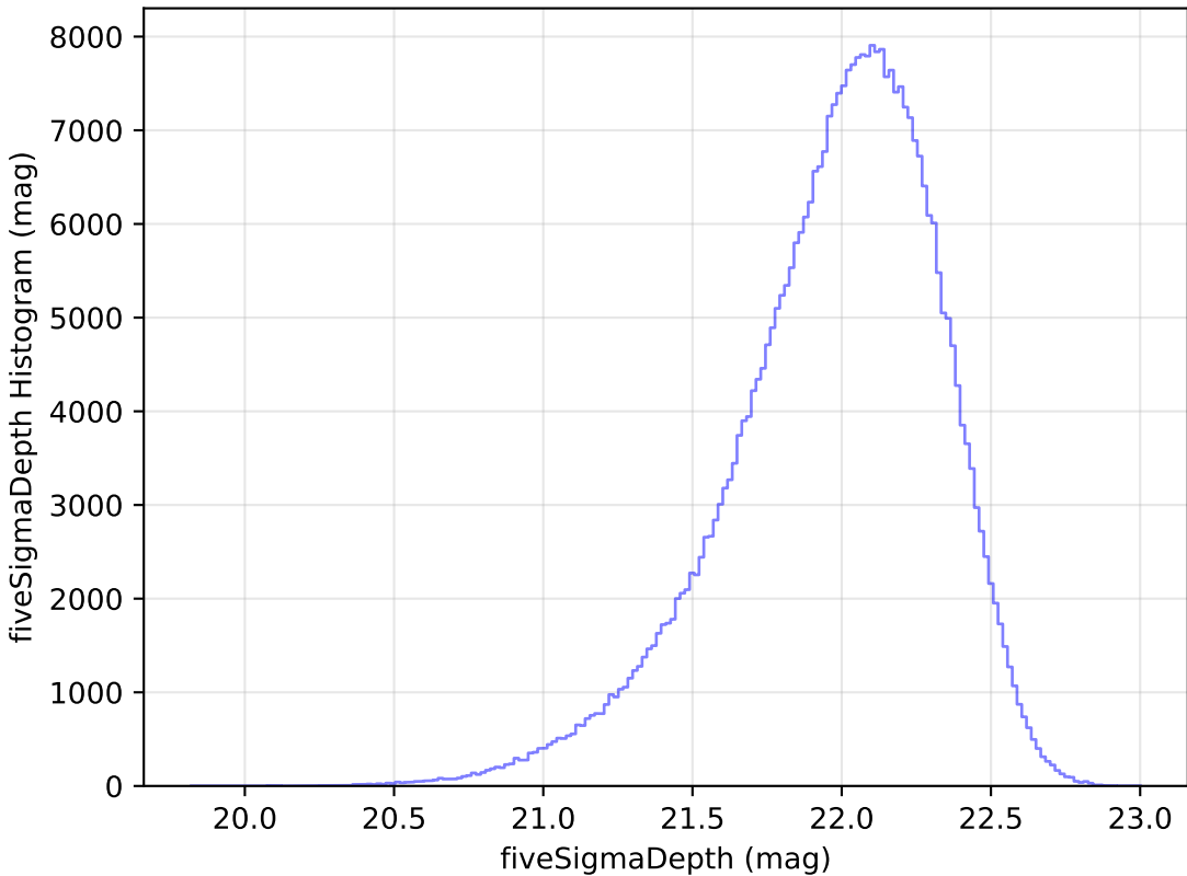
baseline_v3.4_10yrs y: fiveSigmaDepth Histogram
