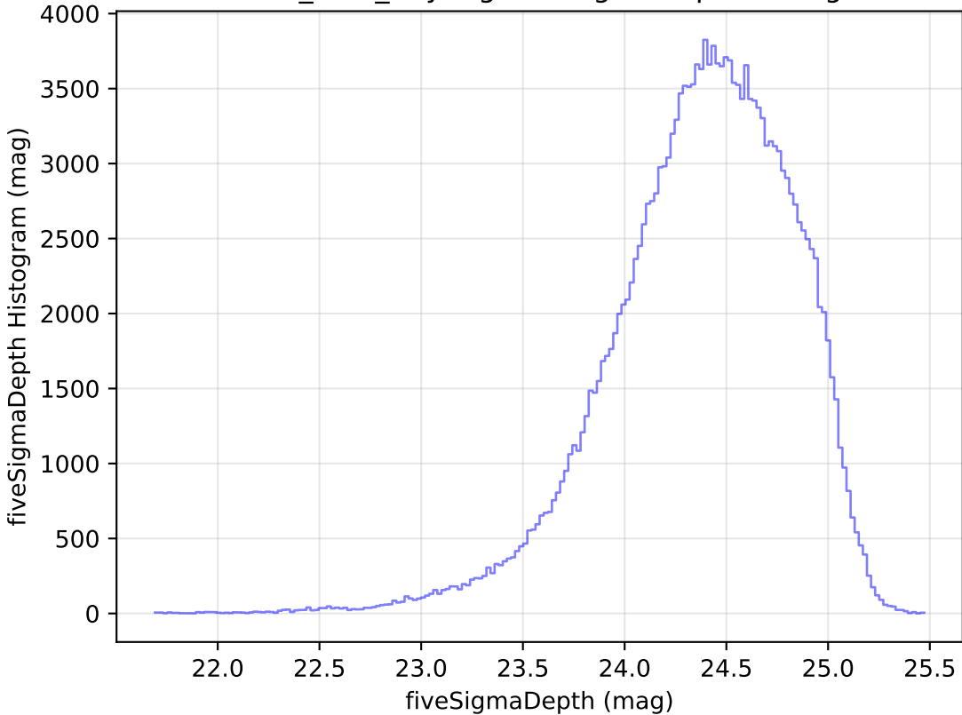
baseline_v3.4_10yrs g: fiveSigmaDepth Histogram
