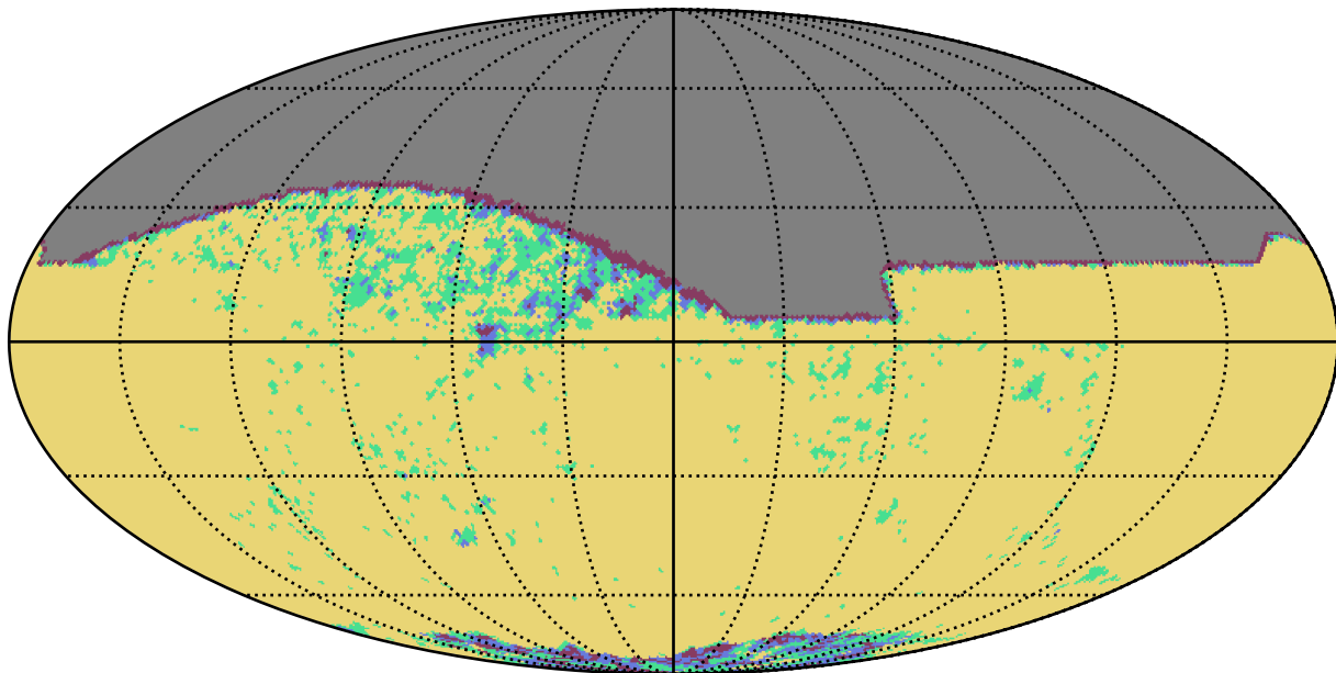
baseline_v3.4_10yrs z band: YearCoverage night
