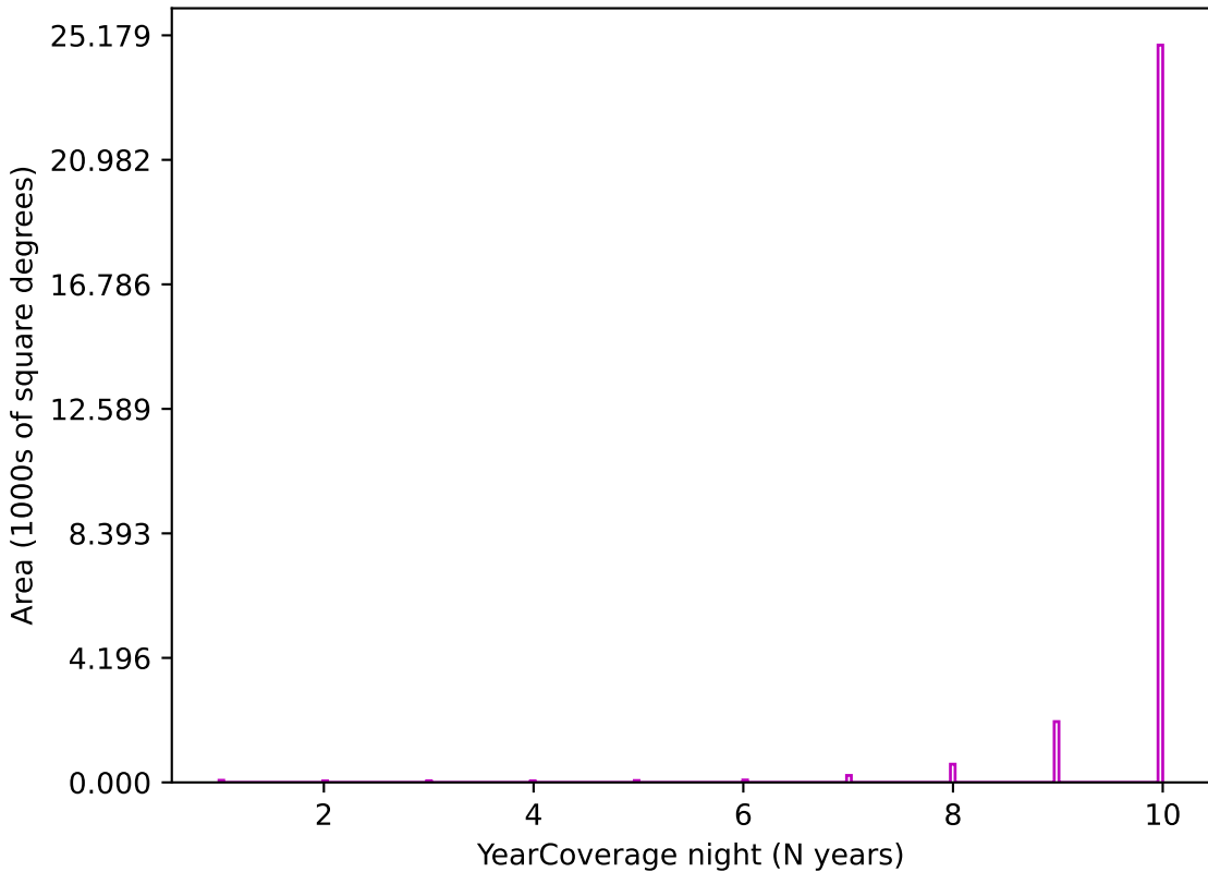
baseline_v3.4_10yrs z band: YearCoverage night
