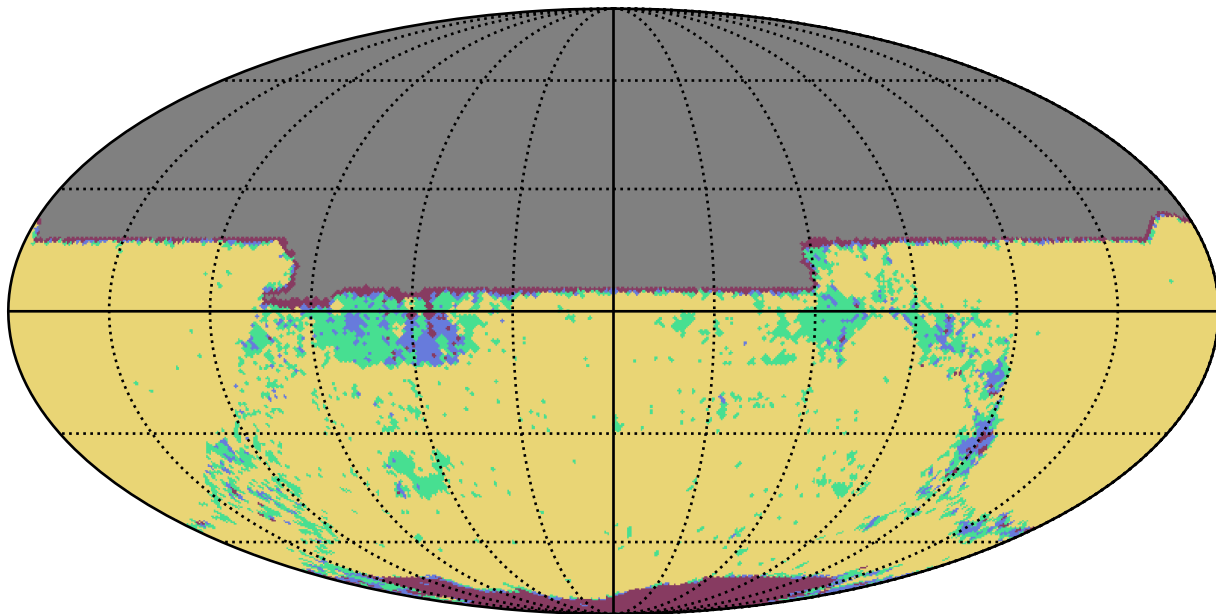
baseline_v3.4_10yrs y band: YearCoverage night
