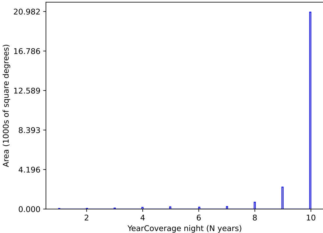
baseline_v3.4_10yrs y band: YearCoverage night
